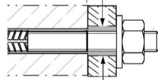
fischer rebar anchor FRA Push through anchor (annular gap filled with mortar)
