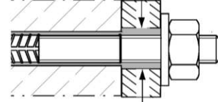
fischer rebar anchor FRA Push through anchor (annular gap filled with mortar)
