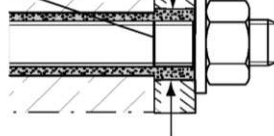
Anchor rod Push through anchor (annular gap filled with mortar)
